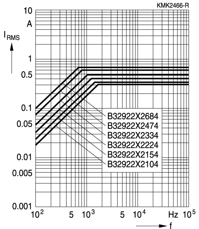
Lead spacing 15 mm
