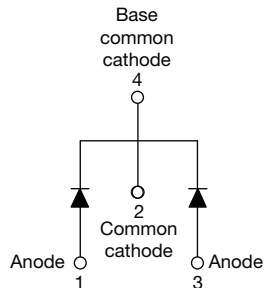
TO-220AB 3L
