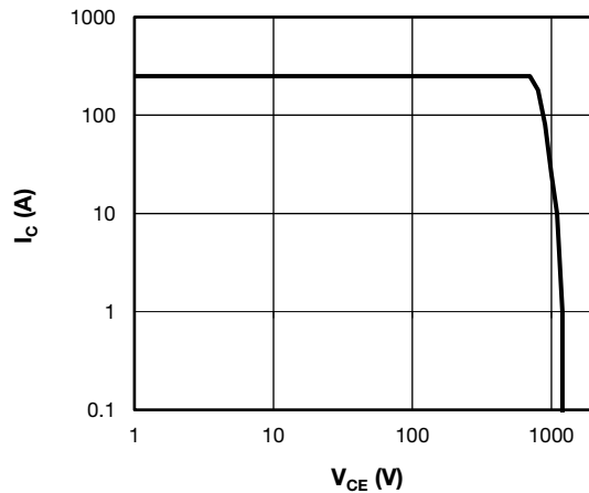
Fig. 16 - Trench IGBT Reverse BIAS SOA T_J = 150\text{ }^\circ\text{C} , I_C = 250\text{A} , R_G = 10\text{ }\Omega , V_{GE} = +15\text{V} , V_{CC} = 700\text{V} , V_p = 1200\text{V}
