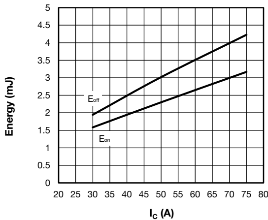
Fig. 7 - Typical Trench IGBT Energy Loss vs. I_C (with Antiparallel Diode) T_J = 125\text{ }^\circ\text{C} , V_{CC} = 600\text{ V} , R_g = 4.7\text{ }\Omega , V_{GE} = +15\text{V}/-15\text{V} , L = 500\text{ }\mu\text{H}
