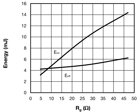
Fig. 9 - Typical Trench IGBT Energy Loss vs. R_g (with Antiparallel Diode) T_J = 125\text{ }^\circ\text{C} , V_{CC} = 600\text{ V} , I_C = 75\text{ A} , V_{GE} = +15\text{V}/-15\text{V} , L = 500\text{ }\mu\text{H}
