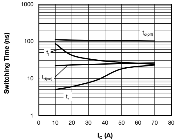
Fig. 8 - Typical Trench IGBT Switching Time vs. I_c (with Antiparallel Diode) T_J = 125\text{ °C} , V_{CC} = 300\text{ V} , R_g = 4.7\ \Omega , V_{GE} = +15\text{ V}/-15\text{ V} , L = 500\ \mu\text{H}
