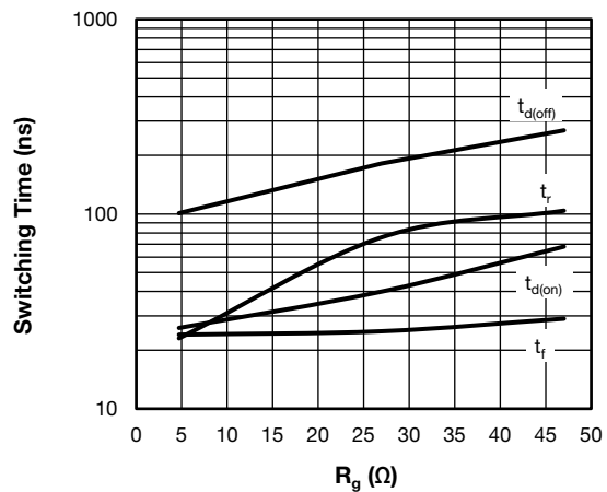
Fig. 10 - Typical Trench IGBT Switching Time vs. R_g (with Antiparallel Diode) T_J = 125\text{ °C} , V_{CC} = 300\text{ V} , I_c = 70\text{ A} , V_{GE} = +15\text{ V}/-15\text{ V} , L = 500\ \mu\text{H}
