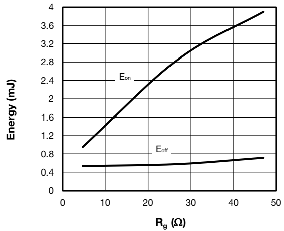
Fig. 9 - Typical Trench IGBT Energy Loss vs. R_g (with Antiparallel Diode) T_J = 125\text{ °C} , V_{CC} = 300\text{ V} , I_c = 70\text{ A} , V_{GE} = +15\text{ V}/-15\text{ V} , L = 500\ \mu\text{H}
