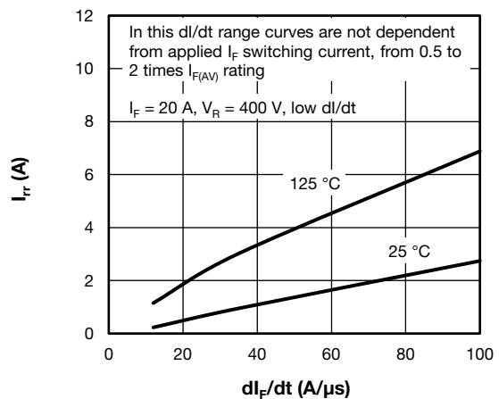
Fig. 12 - Typical Reverse Recovery Current vs. dl_F/dt
