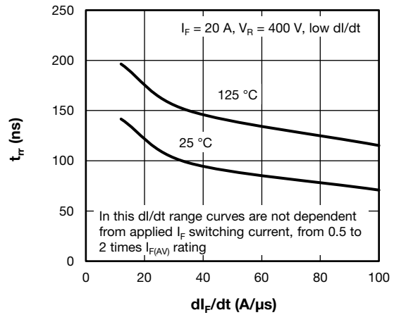
Fig. 10 - Typical Reverse Recovery Time vs. dl_F/dt
