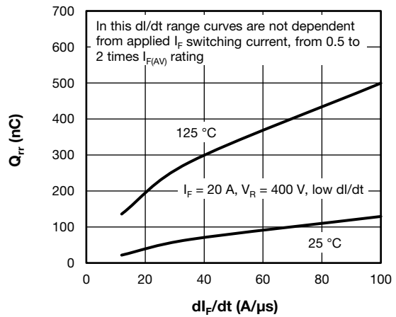
Fig. 11 - Typical Reverse Recovery Charge vs. dl_F/dt
