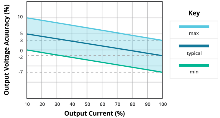
OUTPUT REGULATION CURVE VQA3-S24-D15-S (-Vo)
