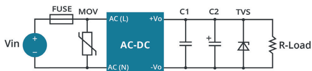
Fig. 1: Typical circuit diagram
