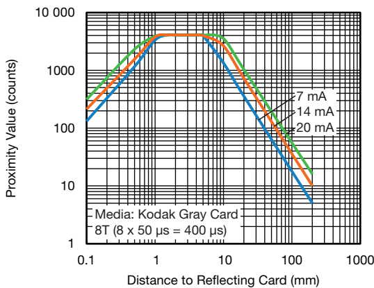
Fig. 7 - Proximity Value vs. Distance; PS_IT = 8T
