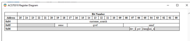
Figure 19: ACS70310 Register Diagram
