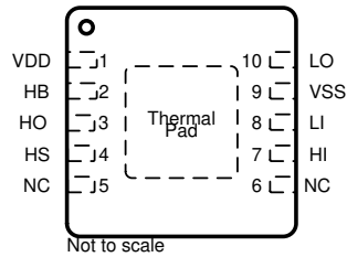
Figure 5-3. DPR Package 10-Pin SON Top View
