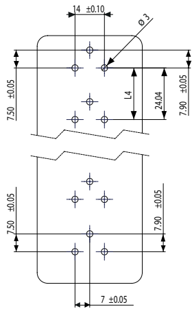
Drilling diagram for PCB terminals: L individua andl N/PE bussed [mm]
