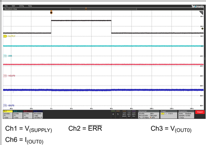
Figure 6-16. Jump Start
