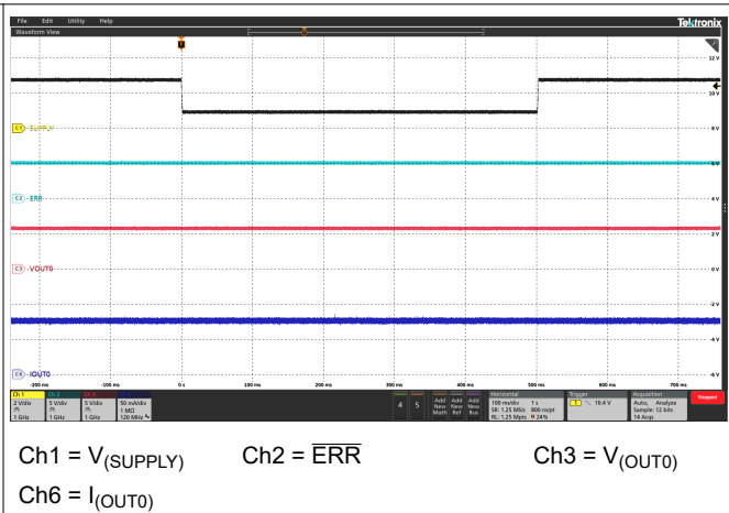
Figure 6-14. Transient Undervoltage
