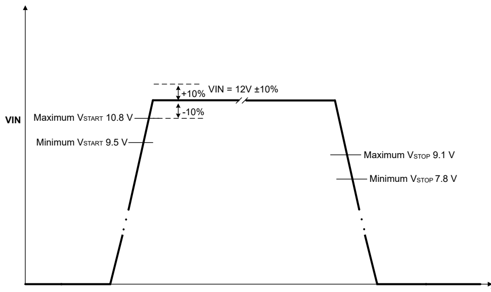
Figure 9-6. Start-Up and UVLO Values for Two-Resistor Configuration With VIN = 12 V
