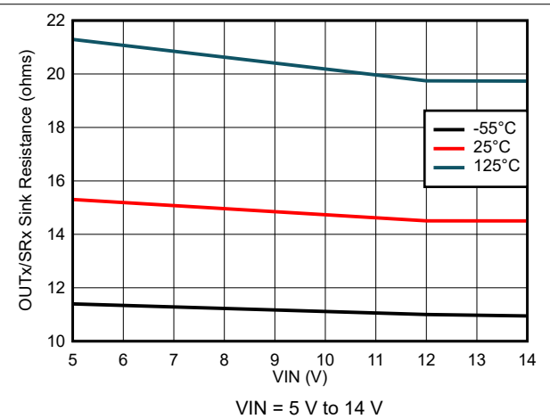
Figure 8-64. Output Sink Resistance Variation
