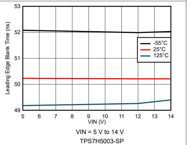
Figure 8-40. Leading Edge Blank Time Variation
