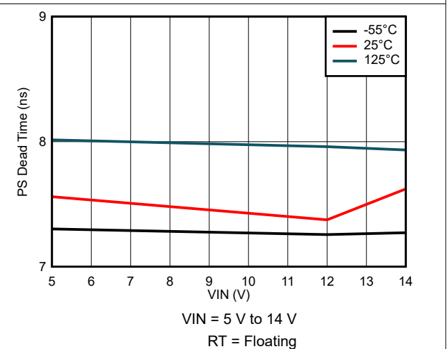
Figure 8-42. PS Dead Time Variation
