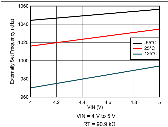
Figure 8-23. Externally Set Frequency Variation
