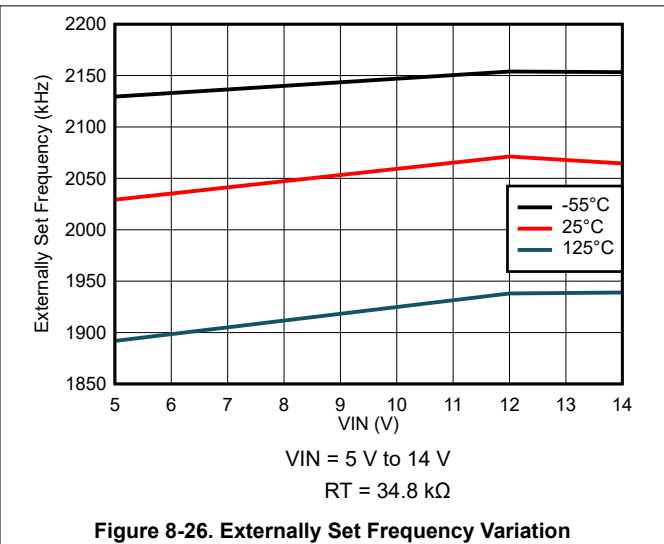
Figure 8-26. Externally Set Frequency Variation
