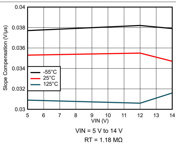
Figure 8-66. Slope Compensation Variation
