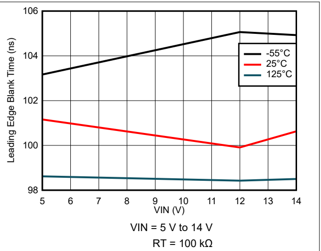
Figure 8-38. Leading Edge Blank Time Variation
