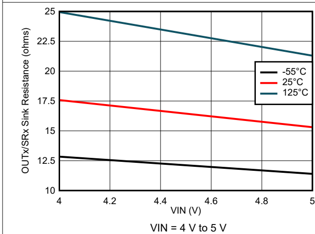
Figure 8-63. Output Sink Resistance Variation
