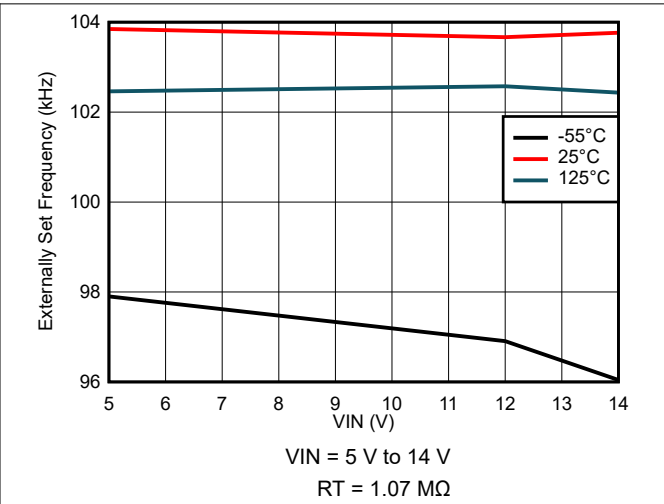
Figure 8-20. Externally Set Frequency Variation
