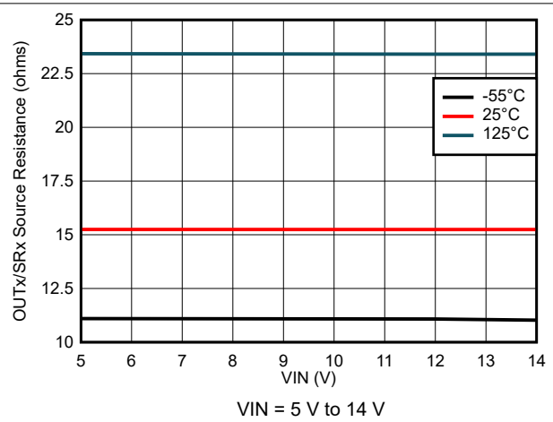
Figure 8-62. Output Source Resistance Variation
