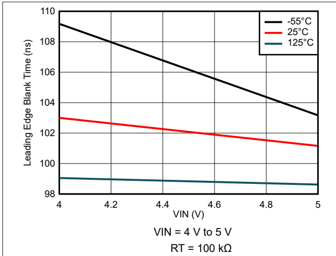
Figure 8-37. Leading Edge Blank Time Variation
