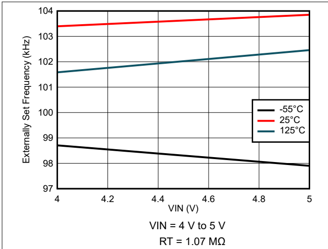
Figure 8-19. Externally Set Frequency Variation
