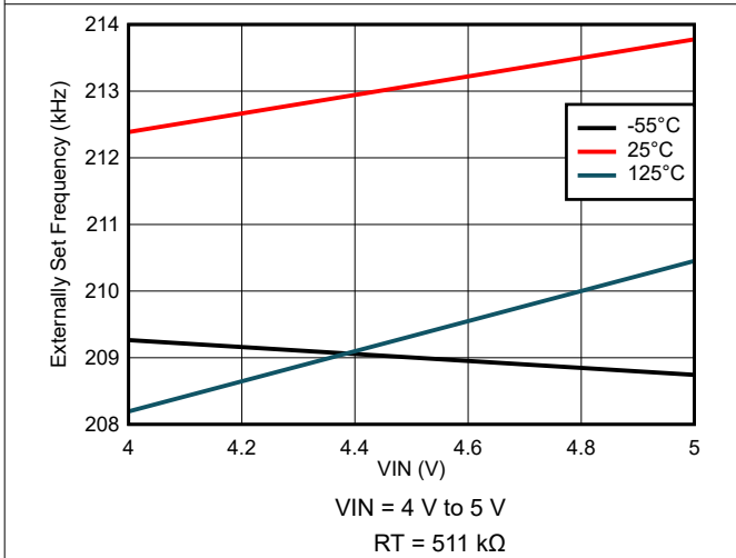
Figure 8-21. Externally Set Frequency Variation
