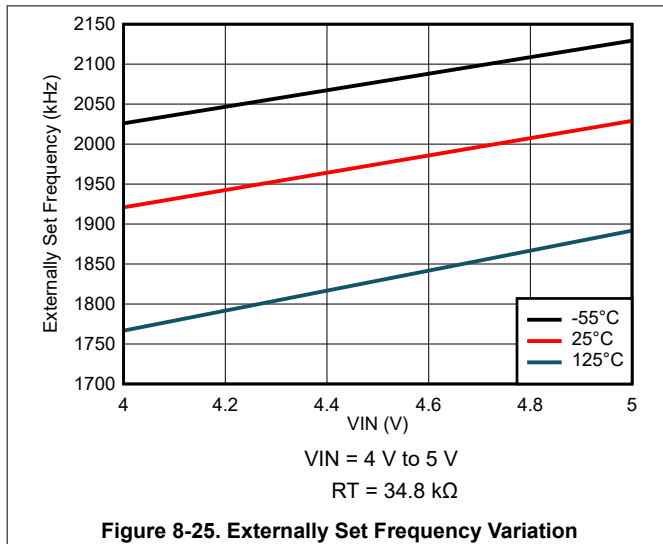
Figure 8-25. Externally Set Frequency Variation
