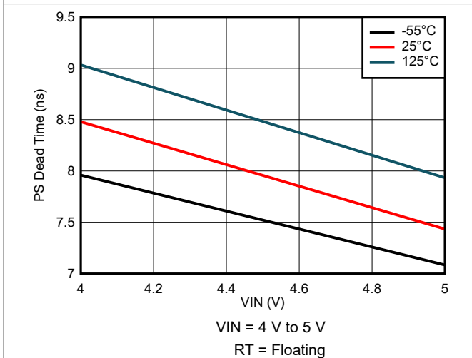
Figure 8-41. PS Dead Time Variation
