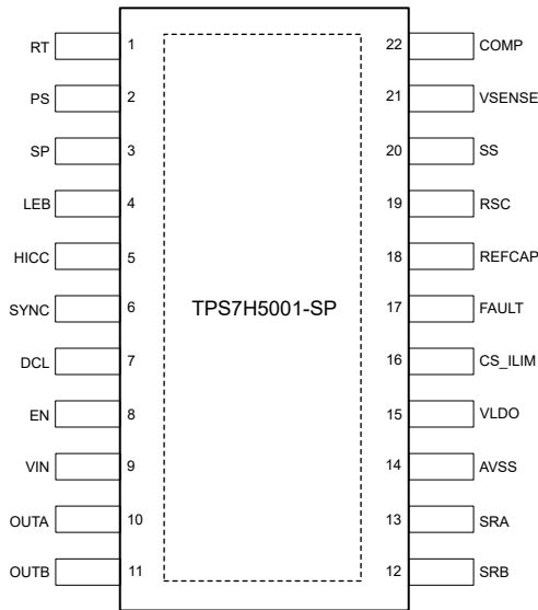
Figure 7-1. TPS7H5001-SP HFT Package 22-Pin CFP With Thermal Pad (Top View)
