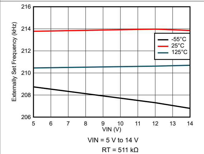
Figure 8-22. Externally Set Frequency Variation
