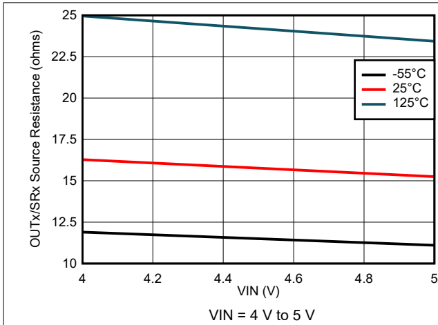
Figure 8-61. Output Source Resistance Variation
