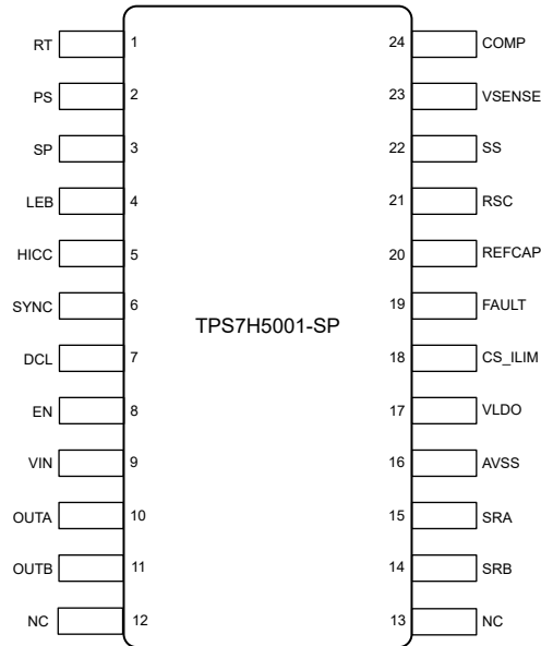
Figure 7-5. TPS7H5001-SP PW Package 24-Pin TSSOP (Top View)
