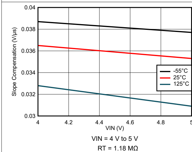
Figure 8-65. Slope Compensation Variation
