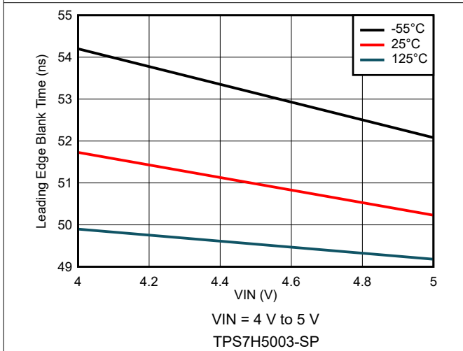
Figure 8-39. Leading Edge Blank Time Variation
