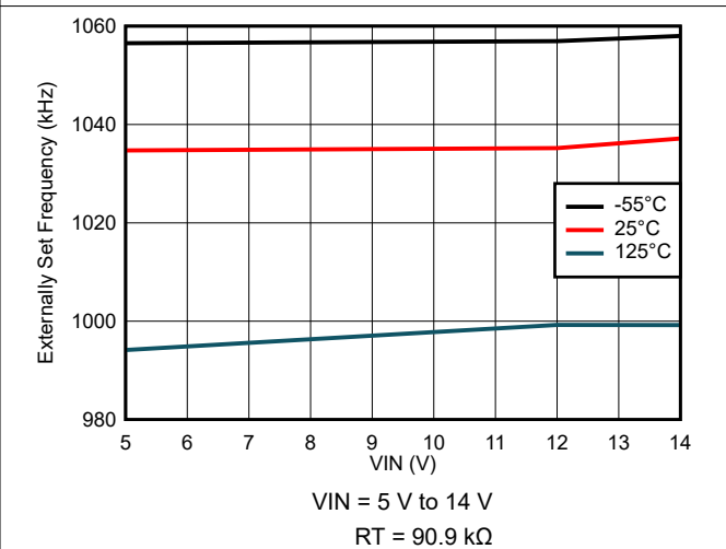
Figure 8-24. Externally Set Frequency Variation
