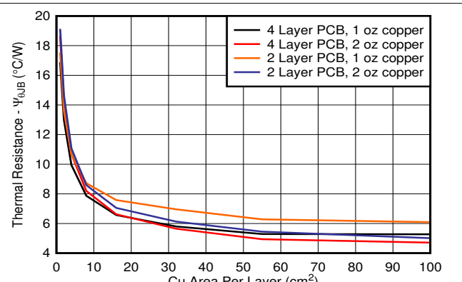
Figure 8-5. \psi_{JB} vs Copper Area (KVU Package)
