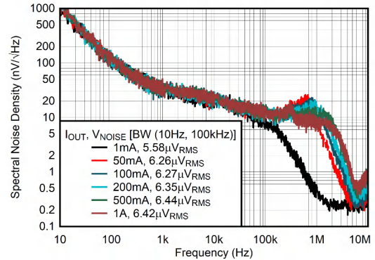
Figure 6-28. Output Noise vs Frequency and I_{OUT}
