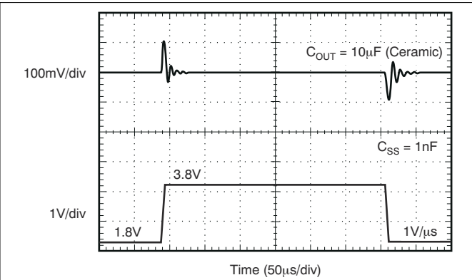
Figure 6-19. V_{IN} Line Transient
