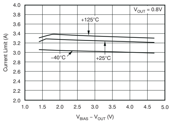
Figure 8-11. Current Limit vs ( V_{BIAS} - V_{OUT} )
