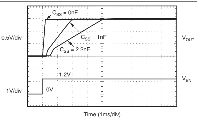
Figure 8-6. Turn-On Response
