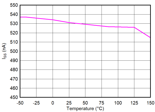
Figure 6-39. Soft-Start Charging Current (I SS ) vs Temperature (T J )
