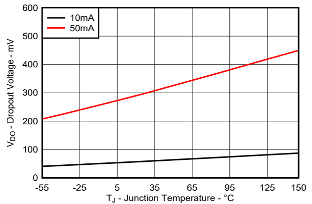
Figure 6-14. Dropout Voltage vs Junction Temperature for New Chip
