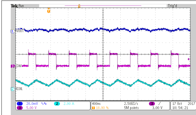
I_{OUT} = 1.0 \text{ A} TPS62824/5/6/7 Figure 9-33. PWM Operation
