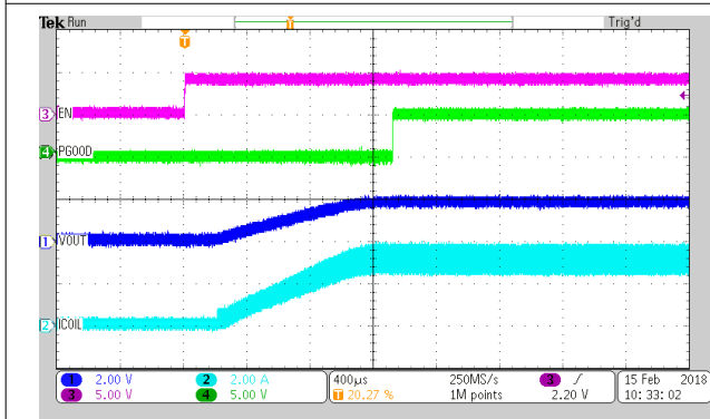
Load = 0.6 \Omega TPS62825/6/7 Figure 9-37. Start-Up With Load
