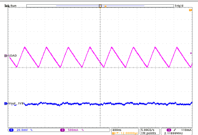
No load TPS62824A/5A/6A/7A Figure 9-36. PWM Operation at F-PWM
