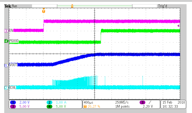
TPS62824/5/6/7 Figure 9-38. Start-Up With No Load
