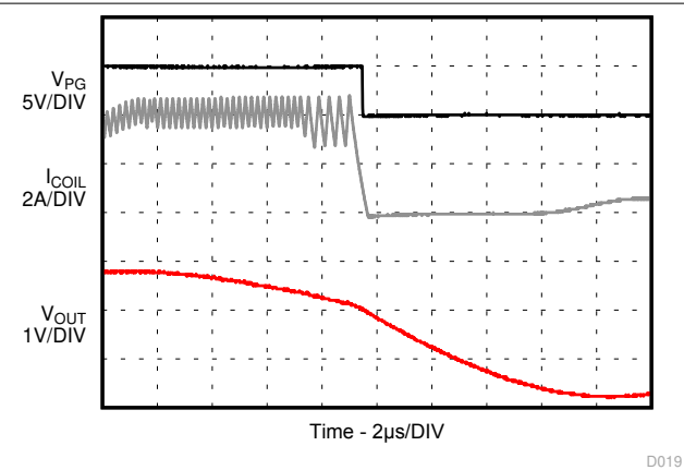
I_{OUT} = 1 \text{ A} TPS6282x
