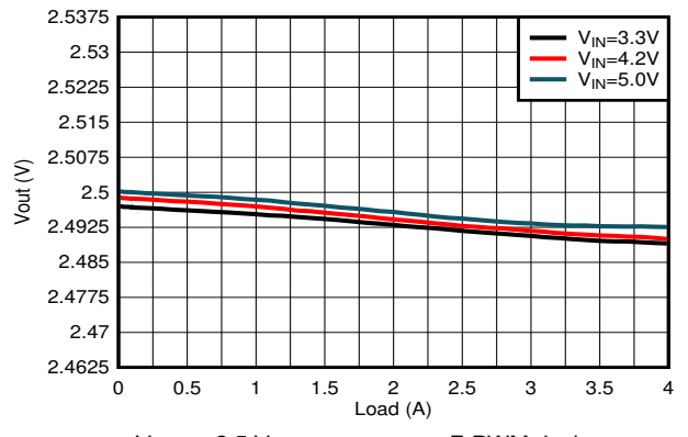
Figure 9-18. Load Regulation
