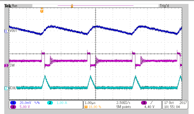
I_{OUT} = 0.1 \text{ A} TPS62824/5/6/7 Figure 9-34. PSM Operation
