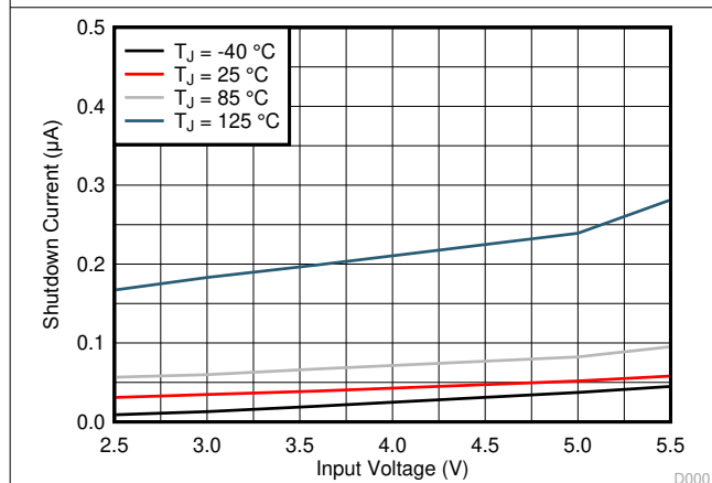
Figure 7-3. Shutdown Current
