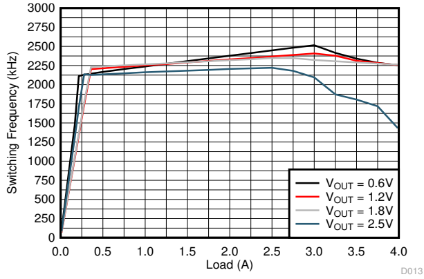
V_{IN} = 3.3\text{ V} TPS62827 Figure 9-27. Switching Frequency
