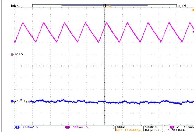
I_{OUT} = 1.0 \text{ A} TPS62824A/5A/6A/7A Figure 9-35. PWM Operation at F-PWM
