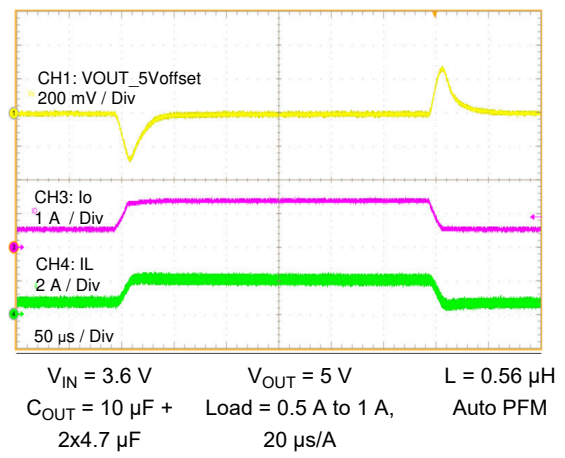
Figure 9-7. Load Transient
