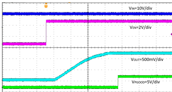
Figure 8-6. Start-Up Relative to EN Rising, Time = 2\ \text{ms}/\text{div}
