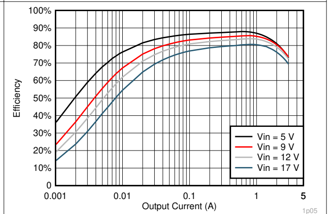
Figure 7-10. V_{OUT} = 1.05 V Efficiency, L = 1.2 \mu H
