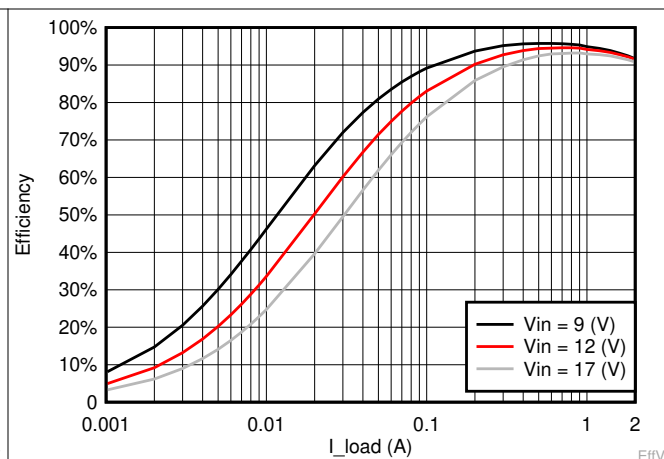
Figure 7-14. V_{OUT} = 5 V Efficiency, L = 4.7 \mu H
