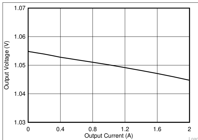
Figure 9-2. Load Regulation with Different Loading
