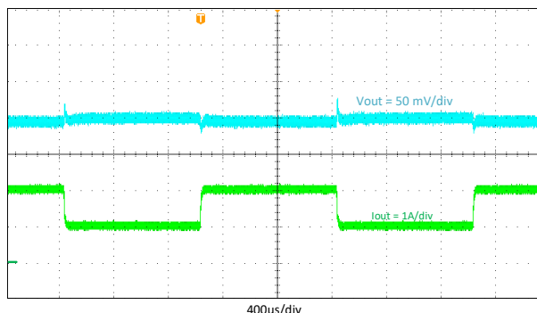
Figure 9-9. Transient Response, 1 to 2 A
