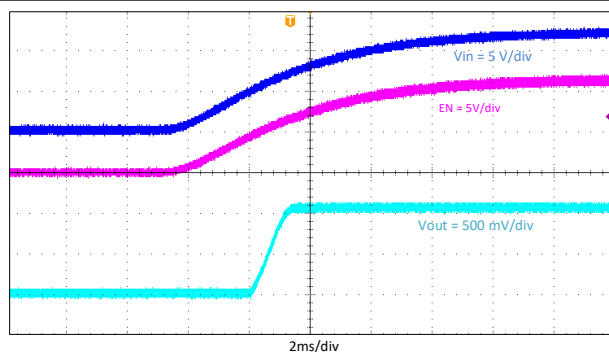
Figure 9-10. Start-Up Relative to V_{IN}
