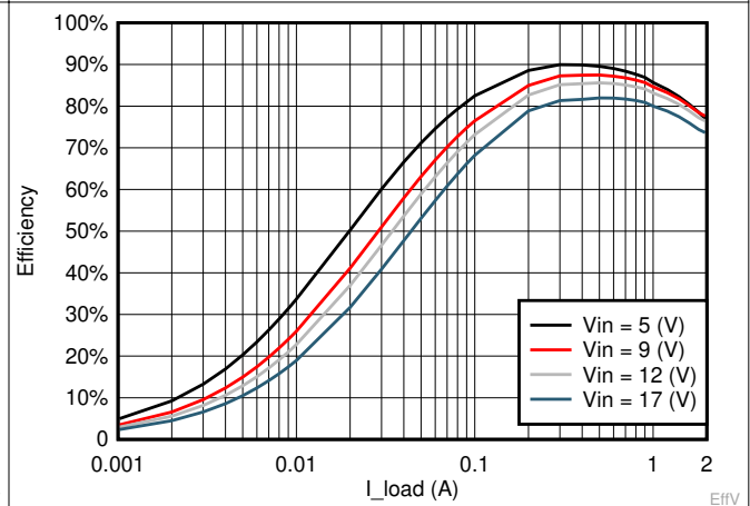
Figure 7-10. V_{OUT} = 1.05 V Efficiency, L = 2.2 \mu\text{H}
