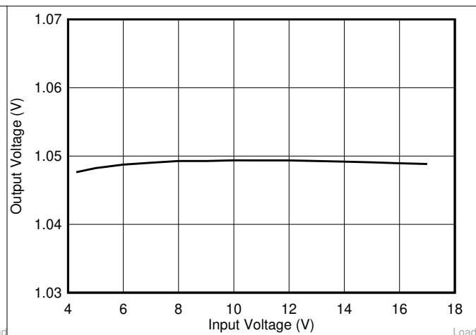
Figure 9-3. Load Regulation with Different Input Voltage
