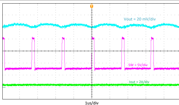
Figure 9-5. Output Voltage Ripple, I_{out} = 0.2 A
