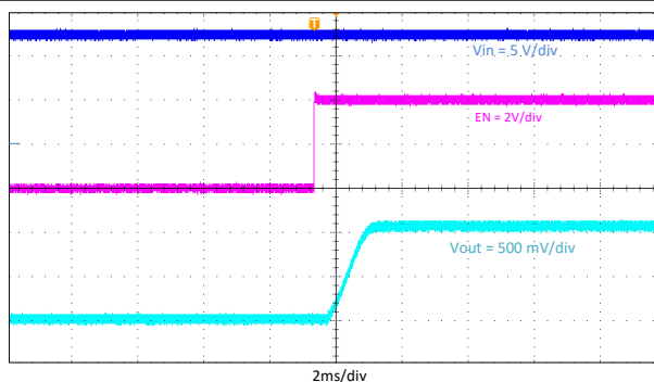
Figure 9-11. Start-Up Relative to EN
