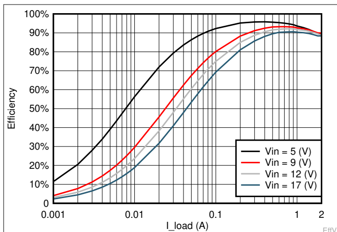
Figure 7-13. V_{OUT} = 3.3 V Efficiency, L = 3.3 \mu H
