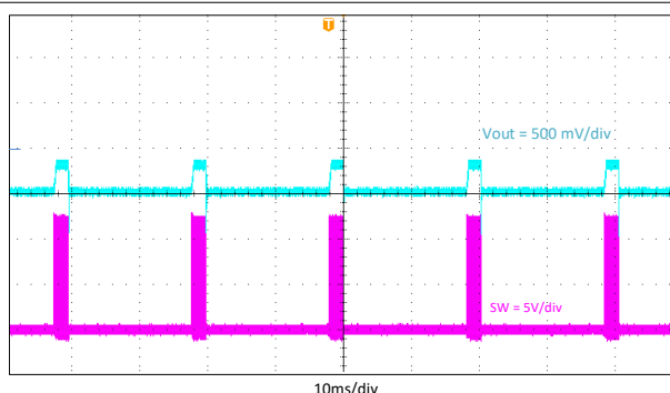
Figure 9-7. Hiccup, I_{out} = 5 A
