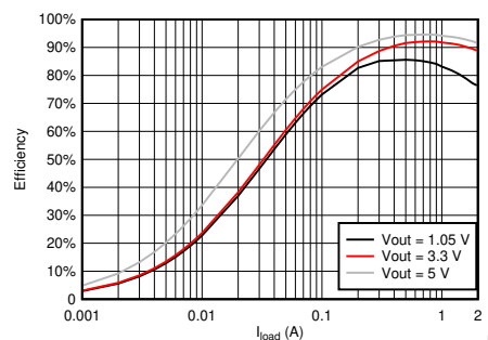
TPS562207S Efficiency
