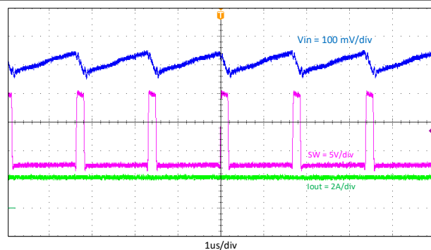
Figure 9-4. Input Voltage Ripple
