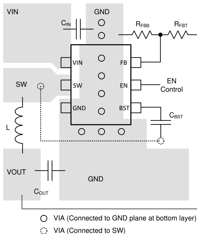
Figure 11-1. TPS562207S Layout
