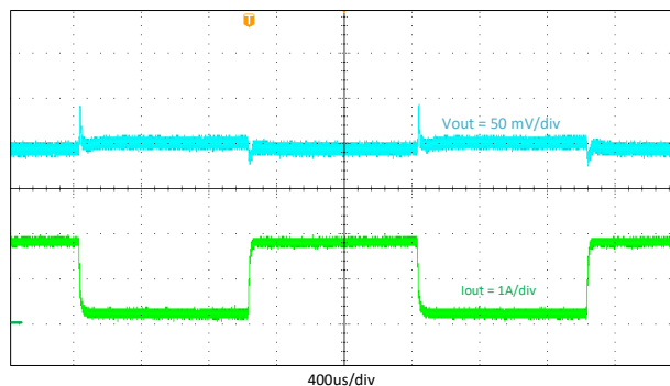
Figure 9-8. Transient Response, 0.2 to 1.8 A
