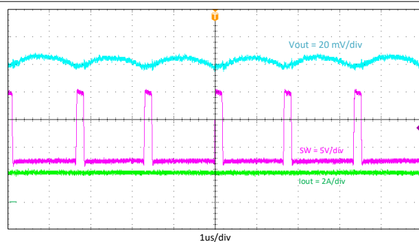
Figure 9-6. Output Voltage Ripple, I_{out} = 2 A
