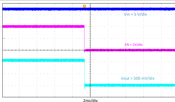
Figure 9-13. Shutdown Relative to EN
