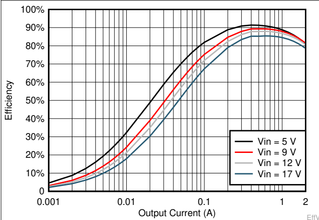
Figure 7-11. V_{OUT} = 1.5 V Efficiency, L = 2.2 \mu\text{H}
