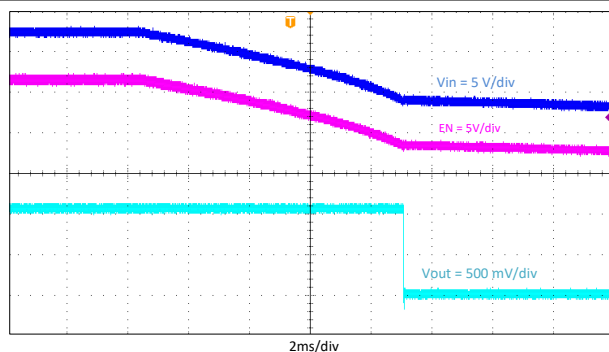
Figure 9-12. Shutdown Relative to V_{IN}
