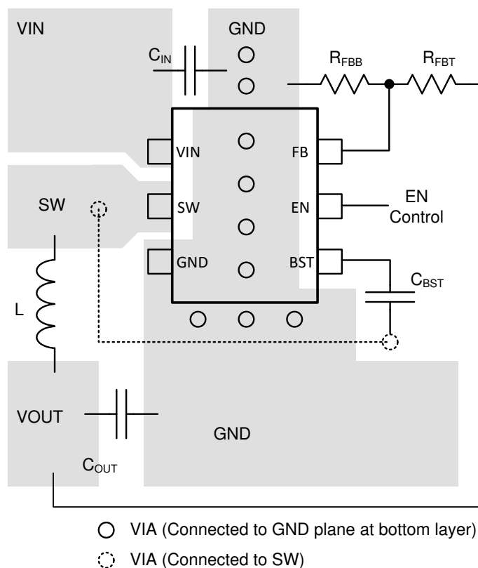
Figure 11-1. TPS562202S Layout
