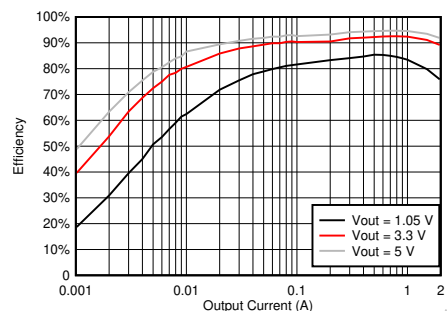
TPS562202S Efficiency
