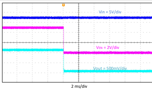
Figure 9-11. Shutdown Relative to EN
