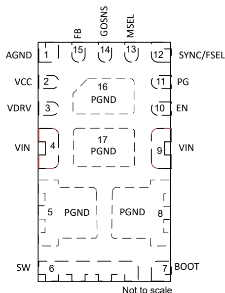
Figure 5-2. 17-Pin WQFN-FCRLF RYS Package (Top View)
