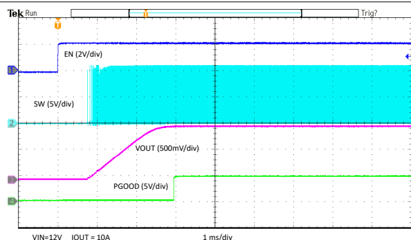
Figure 8-12. EN Start-Up – With Load
