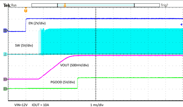
Figure 8-10. EN Start-Up – Measuring SW
