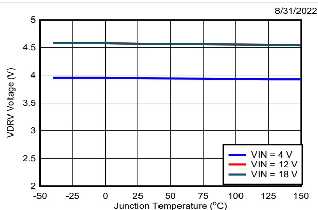
Figure 6-15. VDRV vs Temperature
