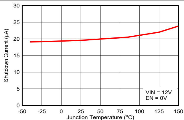
Figure 6-14. Shutdown Supply Current
