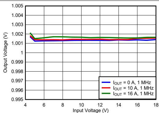
Figure 8-6. Line Regulation
