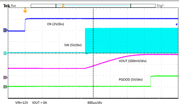
Figure 8-13. EN Start-Up – 0.5-V Prebias
