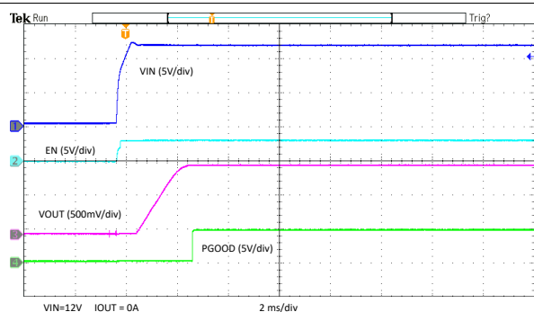
Figure 8-14. VIN Start-Up
