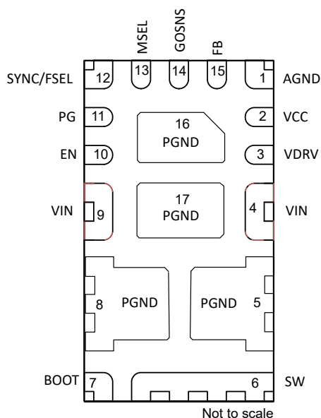
Figure 5-1. 17-Pin WQFN-FCRLF RYS Package (Bottom View)
