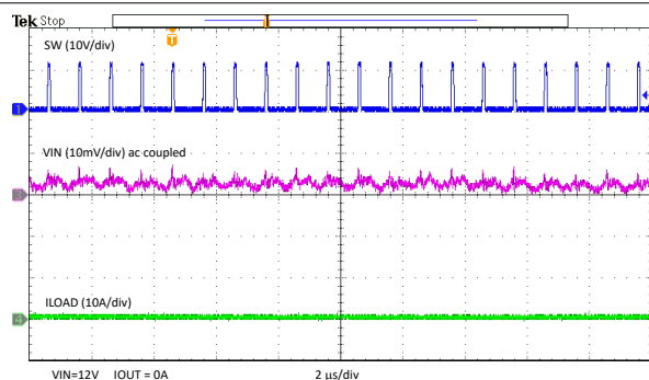
Figure 8-18. Input Ripple – No Load
