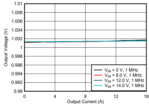
Figure 8-5. Load Regulation
