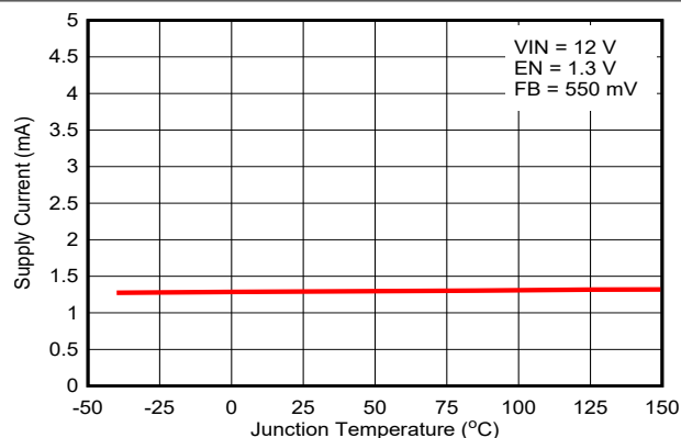
Figure 6-13. Non-Switching Supply Current
