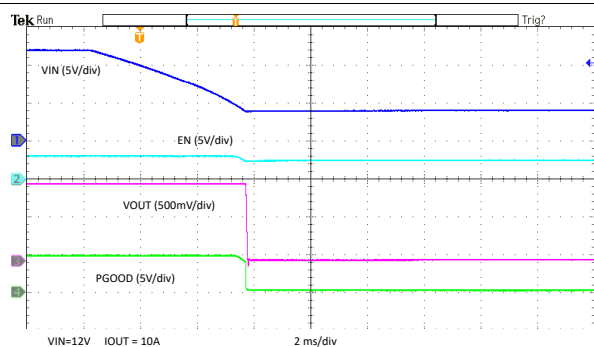
Figure 8-15. VIN Shutdown
