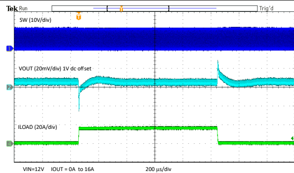
Figure 8-8. Load Transient
