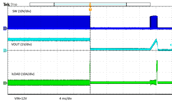
Figure 8-22. Overcurrent Protection – Hiccup and Recover
