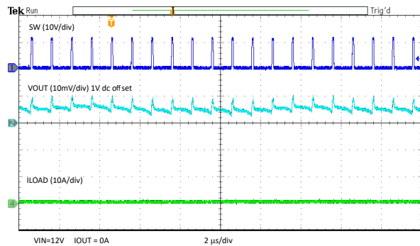
Figure 8-16. Output Ripple – No Load
