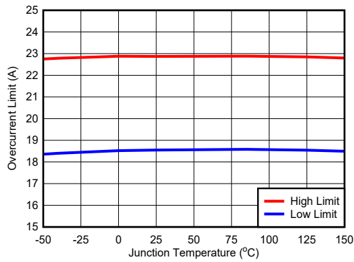
Figure 6-3. Overcurrent Limit
