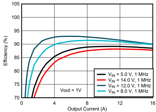
Figure 8-4. Efficiency Curves
