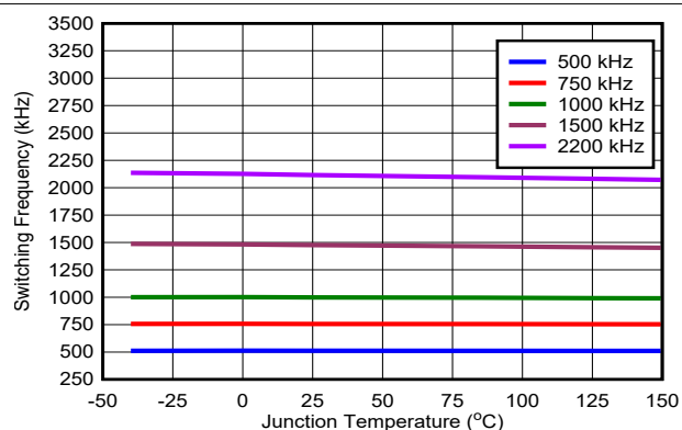
Figure 6-16. Switching Frequency vs Temperature
