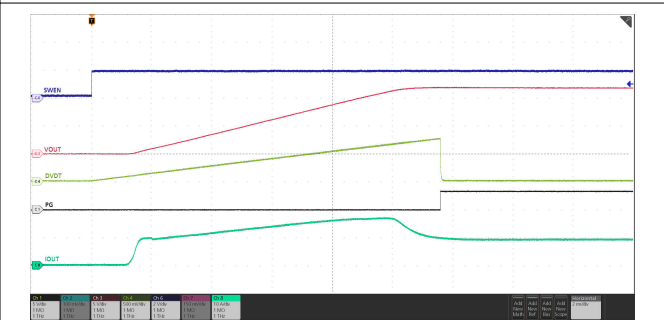
C_{OUT} = 6.8 \text{ mF} , R_{OUT} = 1.2 \Omega , C_{dVdt} = 33 \text{ nF} Figure 7-28. Inrush Current Control with Capacitive and Resistive Load
