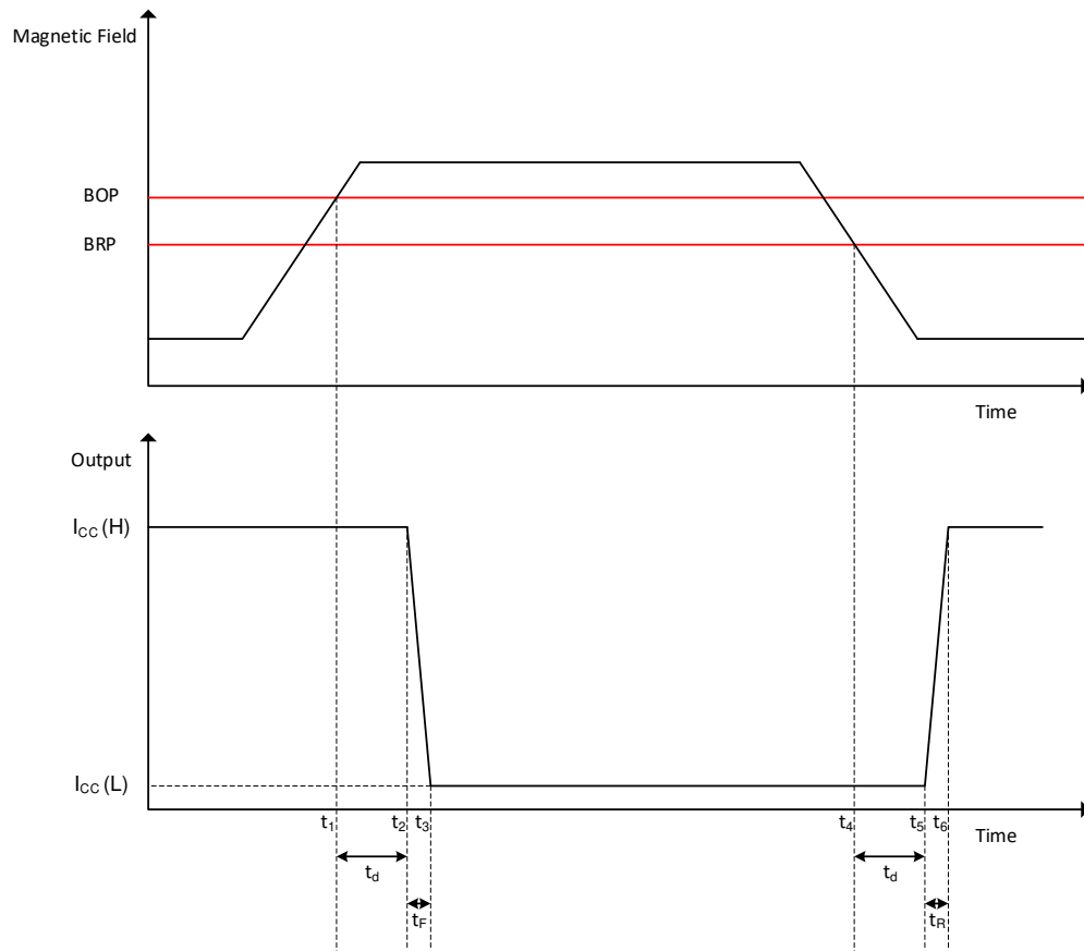
Figure 8-8. Propagation Delay
