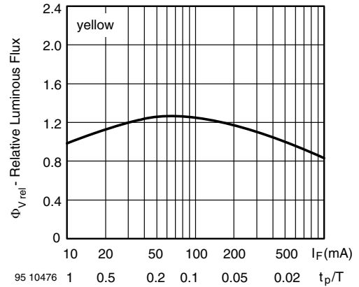
Fig. 7 - Relative Luminous Flux vs. Forward Current/Duty Cycle
