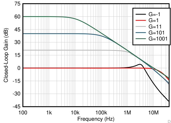
Figure 6-8. Closed-Loop Gain vs Frequency
