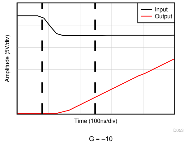
Figure 6-30. Negative Overload Recovery G = -10
