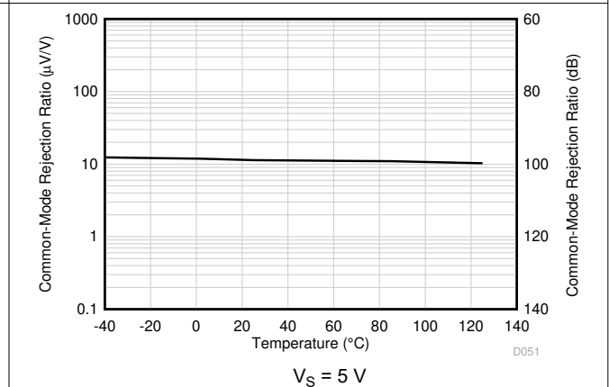
Figure 6-18. CMRR vs Temperature
