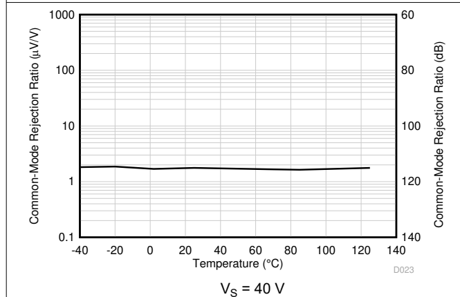
Figure 6-17. CMRR vs Temperature
