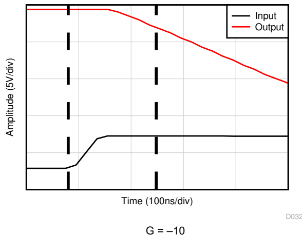
Figure 6-29. Positive Overload Recovery G = -10
