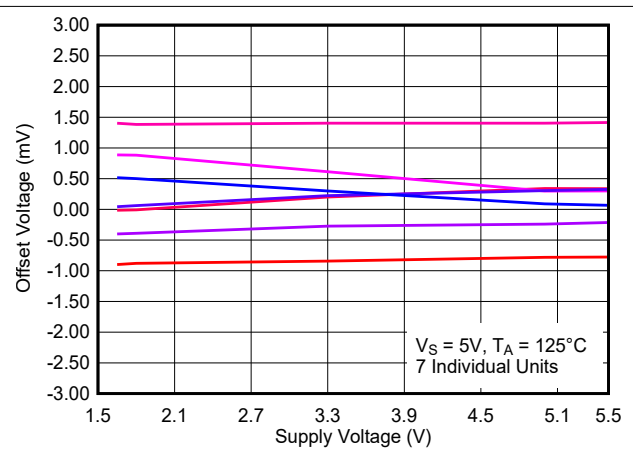
Figure 8-32. Offset Voltage vs. Supply Voltage, 125°C
