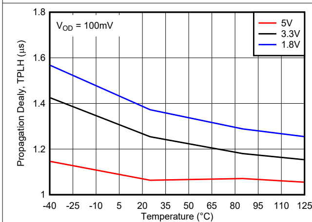
Figure 8-15. Low to High Propagation Delay vs. Temperature
