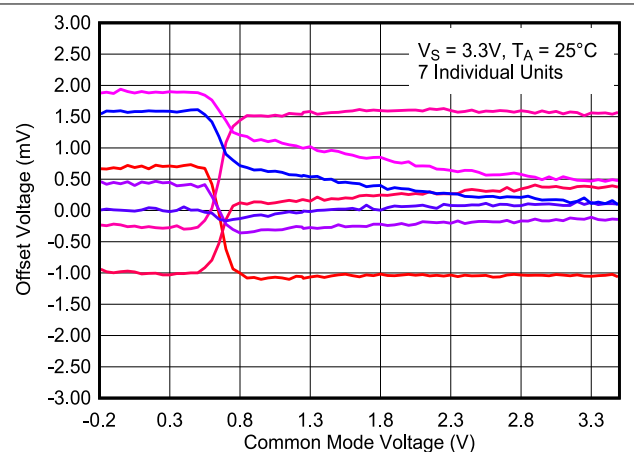
Figure 8-30. Offset Voltage vs. Common Mode Voltage, 3.3 V
