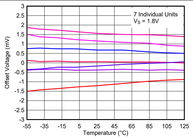
Figure 8-26. Offset Voltage vs. Temperature, 1.8 V
