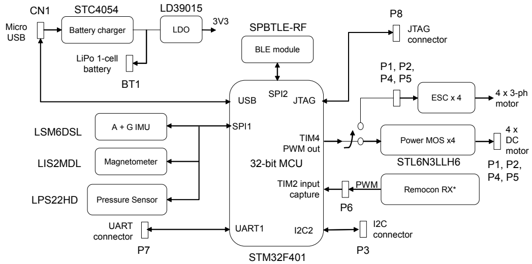
Figure 1. STEVAL-FCU001V1 – block diagram
