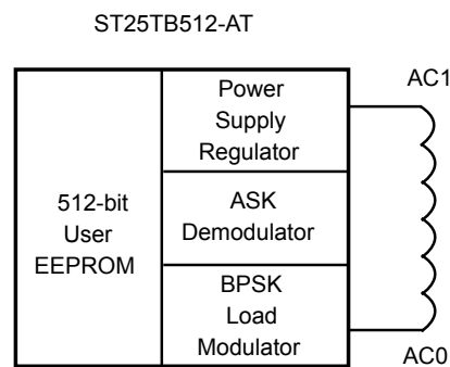
Figure 1. Logic diagram
