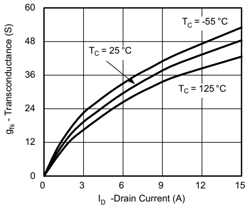
Transconductance
