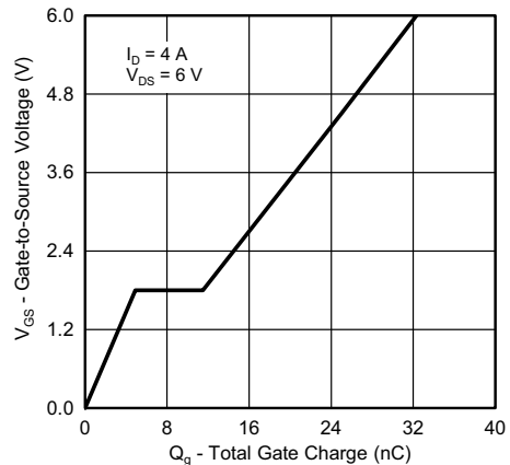
Gate Charge
