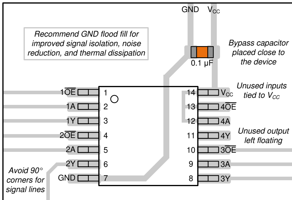
Figure 11-1. Example Layout for the SN74LV4T125-Q1
