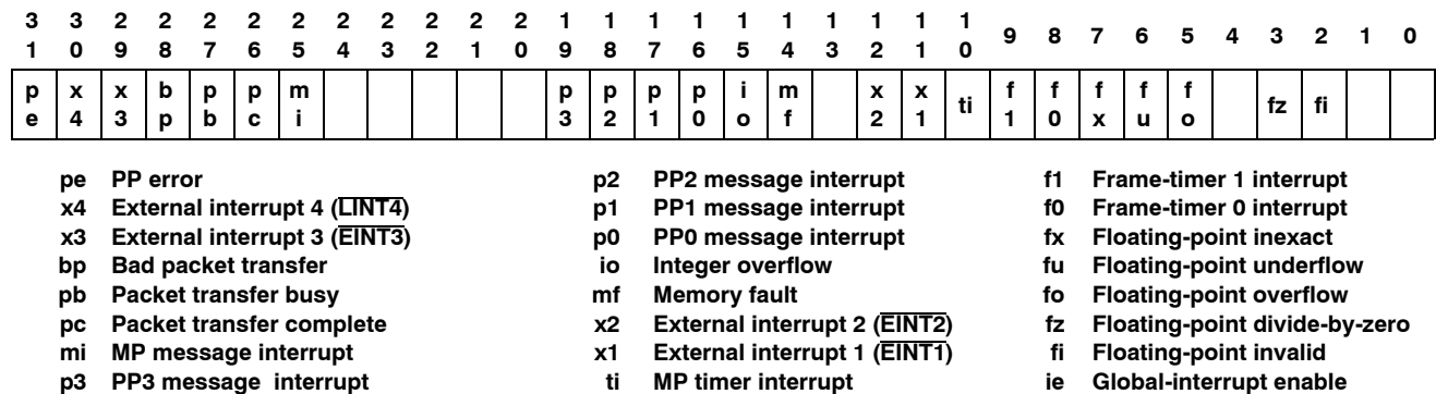
Figure 12. INTPEN Register
