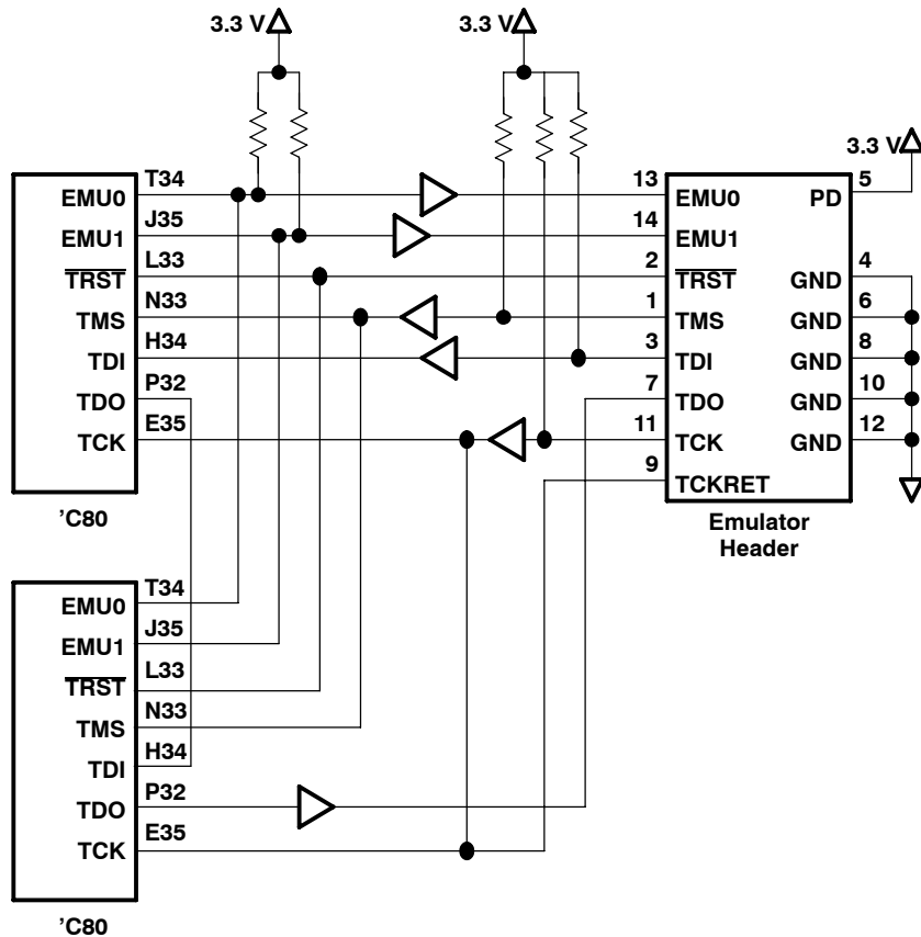
Figure 127. Emulation Header Connections - Multiprocessor Applications
