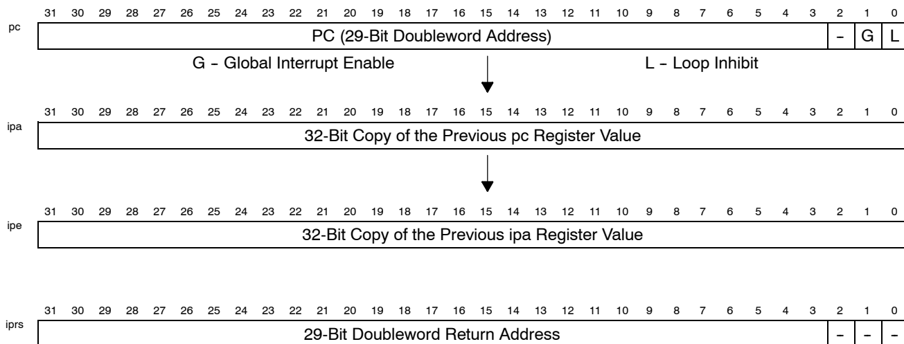
Figure 30. Pipeline Registers
