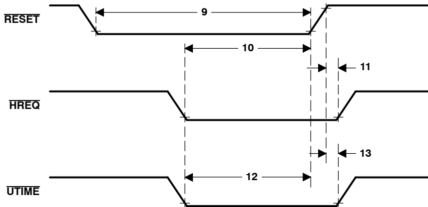
Figure 110. Device-Reset Timing
