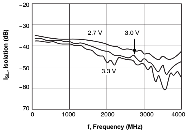
Figure 6. I_{SL} - f
