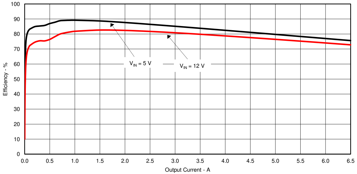
Figure 4-1. TPS54626EVM-608 Efficiency
