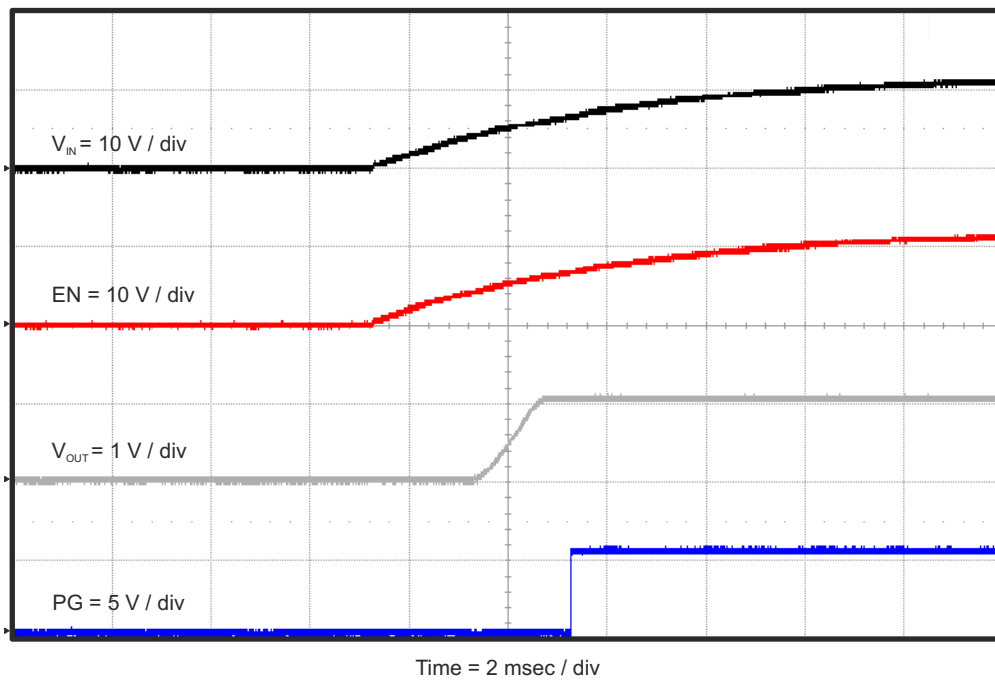
Figure 4-11. TPS54626EVM-608 Start Up Relative to V_{IN}
