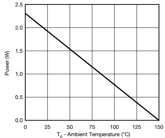
Power, Junction-to-Ambient
