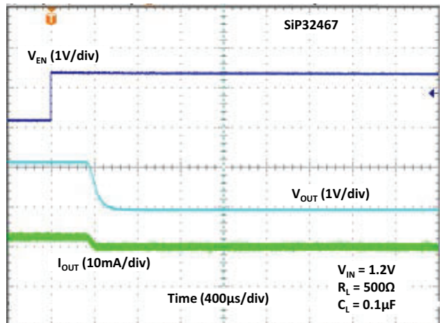
Fig. 27 - Turn-off Time
