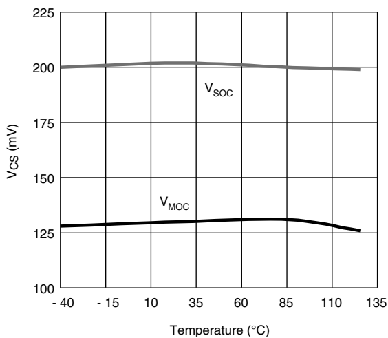
V CS vs. Temperature
