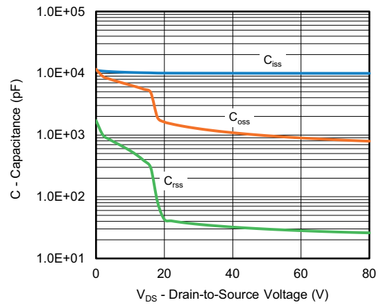
Capacitance
