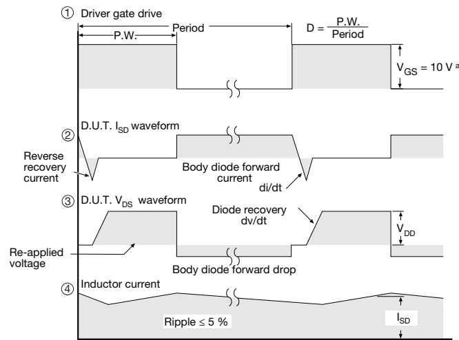
Fig. 20 - For N-Channel
