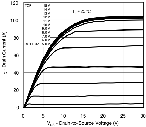
Fig. 1 - Typical Output Characteristics, T C = 150 °C
