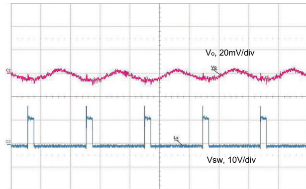
Fig. 55 - Output Ripple, 6 A, t = 1\text{ }\mu\text{s/div} Forced Continuous Conduction Mode
