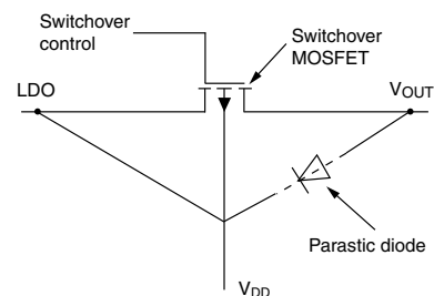
Fig. 12 - Switch-over MOSFET Parasitic Diodes
