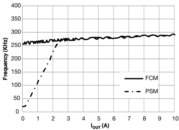
Fig. 9 - Switching Frequency - PSM vs. FCM (V DD = 5 V, V OUT = 1.5 V, V IN = 12 V)
