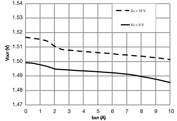
Fig. 11 - Load Regulation - PSM (V DD = 3.3 V, V OUT = 1.5 V)
