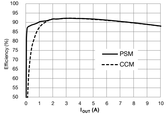
Fig. 4 - Efficiency - PSM vs. CCM ( V_{DD} = 3.3\text{ V} , V_{OUT} = 1.5\text{ V} , V_{IN} = 12\text{ V} )
