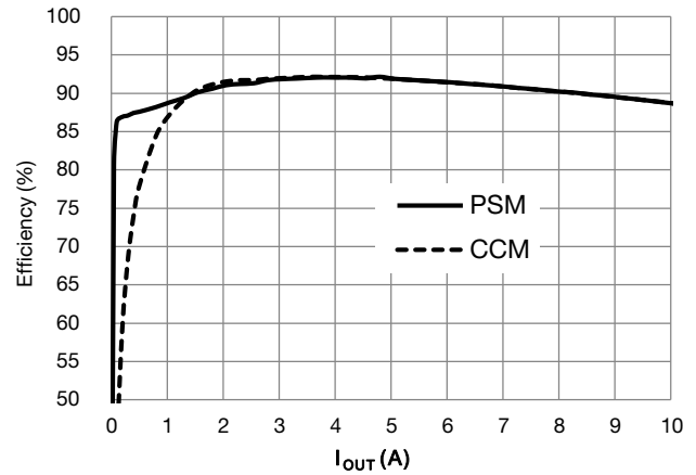
Fig. 5 - Efficiency - PSM vs. CCM ( V_{DD} = 5\text{ V} , V_{OUT} = 1.5\text{ V} , V_{IN} = 12\text{ V} )
