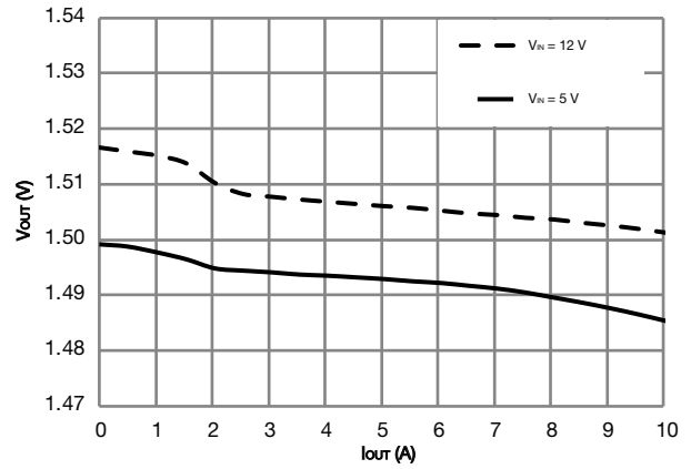
Fig. 10 - Load Regulation - FCM (V DD = 3.3 V, V OUT = 1.5 V)
