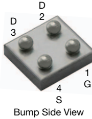
MICRO FOOT® 1.6 x 1.6
