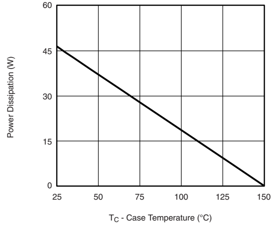
Power, Junction-to-Case
