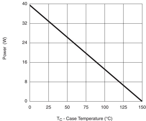
Power, Junction-to-Case
